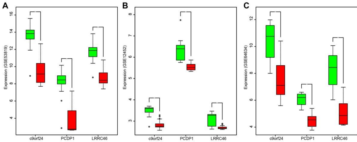
Figure S1 c9orf24, PCDP1 and LRRC46 are poorly expressed in NPC. A-C, the expression of c9orf24, PCDP1 and LRRC46 in gene expression datasets GSE53819, GSE12452 and GSE64634. The abscissa represents gene name, and the ordinate represents gene expression. The green box plot indicates gene expression in non-cancerous tissue specimens, and the red one indicates gene expression in NPC specimens. NPC, nasopharyngeal carcinoma.
