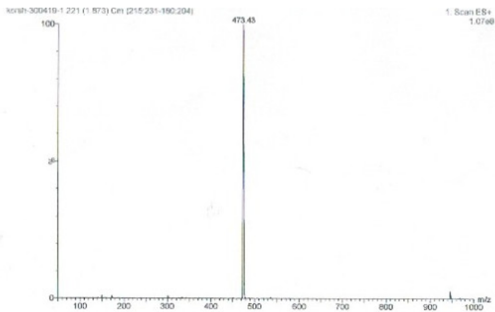
Figure S2. ESI-MS spectra of C10-FL.
