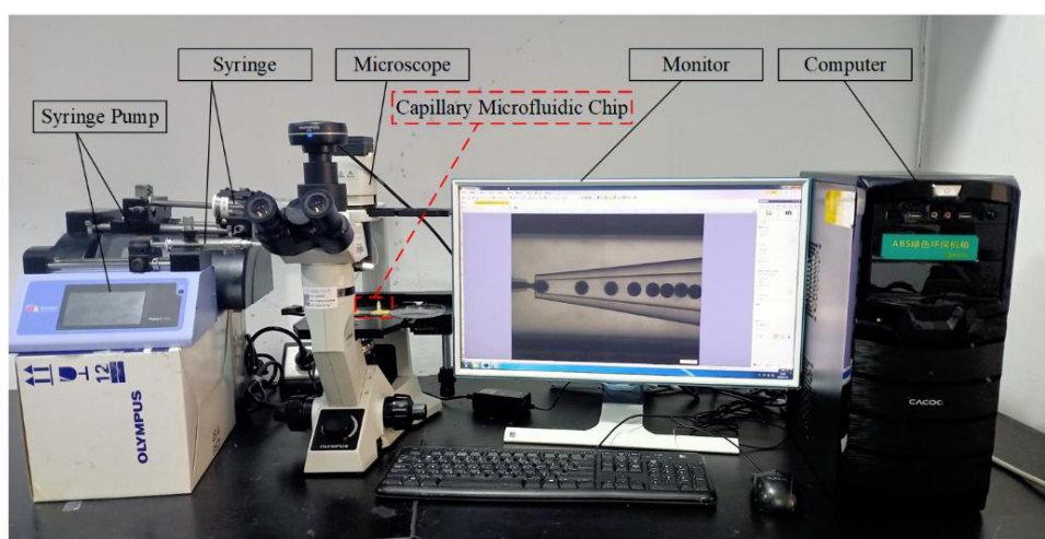
Figure S1. The image of the experimental setup.
