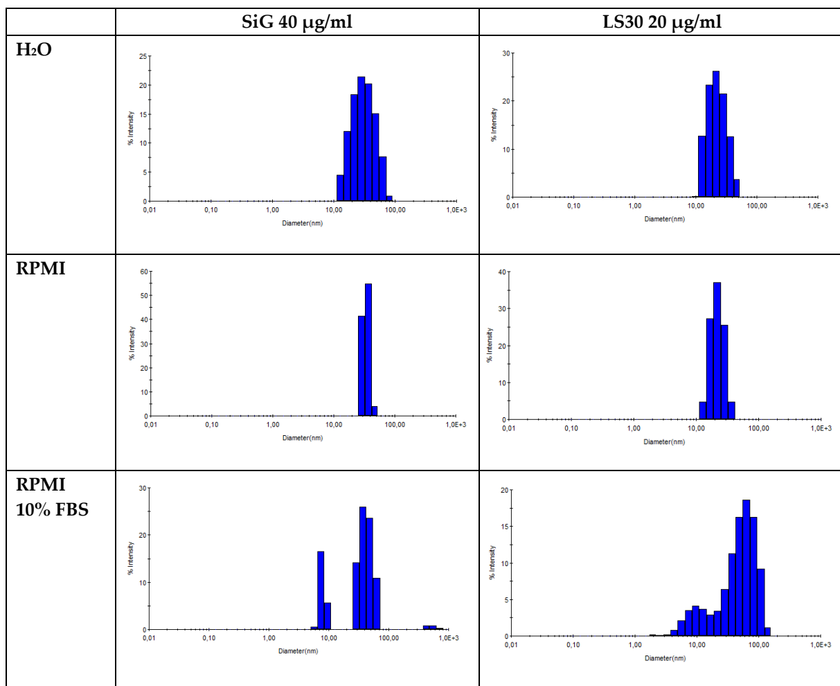
Supplementary table S1: Nano size distribution of silica nanoparticles in water and culture media by DLS. SiG for Sicastar®-greenF, LS30 for Ludox LS30, RPMI for Roswell Park Memorial Institute 1640 medium, FBS for fetal bovine serum. Distribution of intensity of nanoparticle population depending on the diameter, in water and culture media.
