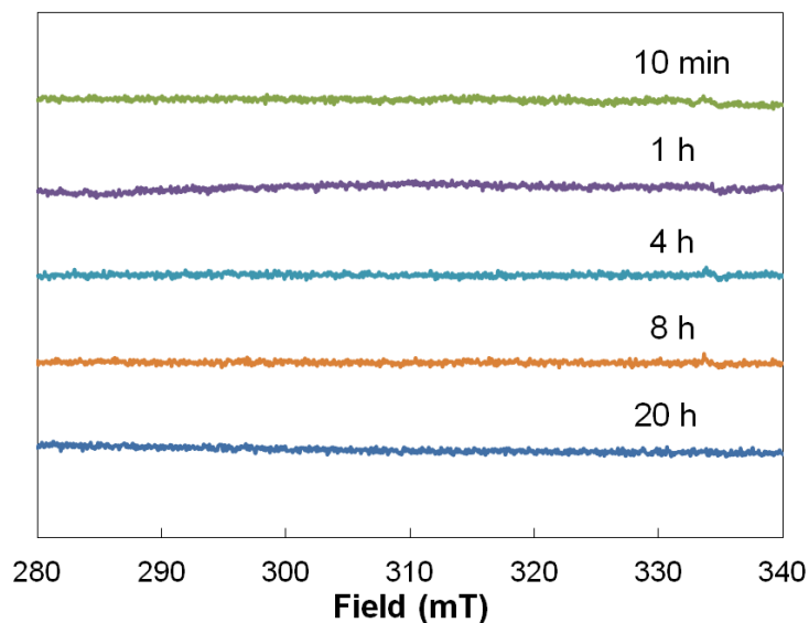
Figure S-1. X-band EPR spectra of the coupling reaction after 10 min, 1 h, 4 h, 8 h, and 20 h. The spectra were collected at \nu = 9.4\text{ GHz} , 2 mW power, and a modulation amplitude of 2 G.
