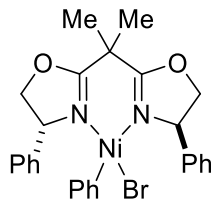
2 Ni II PhBr(Ph-BOX) singlet
