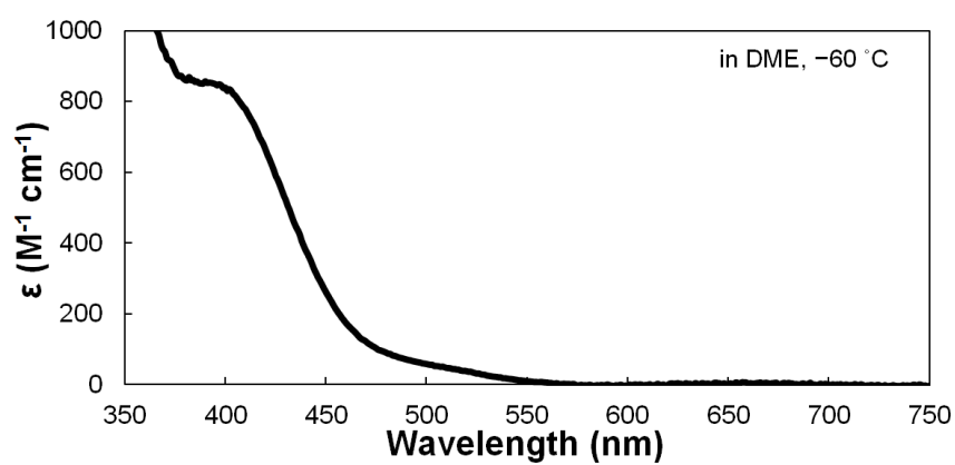
Figure S-8. UV-vis spectrum (DME, -60\text{ }^{\circ}\text{C} ) of ((R,R)\text{-Ph-BOX})\text{Ni}^{\text{I}}\text{Br} ( 3 ).
