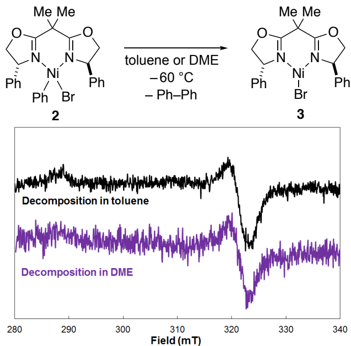
Figure S-4. Stability of Ni II (Ph)Br(Ph-BOX) ( 2 ) at -60 °C after 3 h in toluene (black trace) and in DME (purple trace): X-band EPR spectra. Quantification indicated that the quantity of Ni I Br(Ph-BOX) ( 3 ) was <0.5% in both solvents. The spectra were collected at \nu = 9.4 GHz, 2 mW power, and a modulation amplitude of 2 G.
