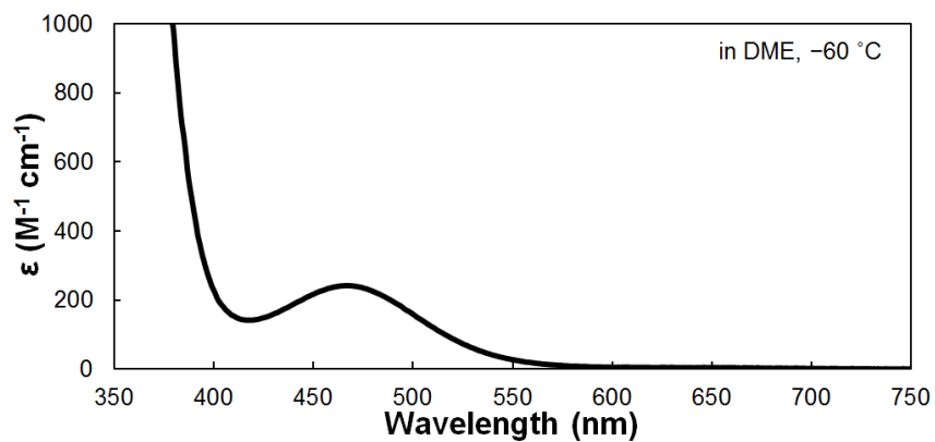
Figure S-7. UV-vis spectrum (DME, -60\text{ }^{\circ}\text{C} ) of ((R,R)\text{-Ph-BOX}^{\text{Ph}})\text{Ni}^{\text{II}}\text{PhBr} ( 2^{\text{Ph}} ).
