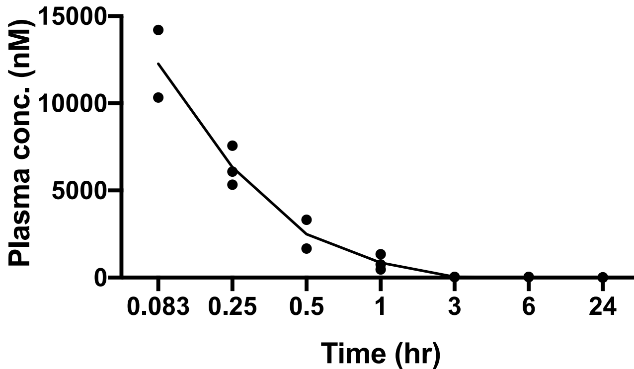
Supplemental Figure 6. Rapid clearance of GNF-9228 in mice. Mice received a single intraperitoneal (IP) injection of 30 mg/kg GNF-9228 suspended in DMSO, and levels of the compound were measured in blood samples collected at the indicated intervals after injection. Blood was sampled from 2-3 mice at each time point.
