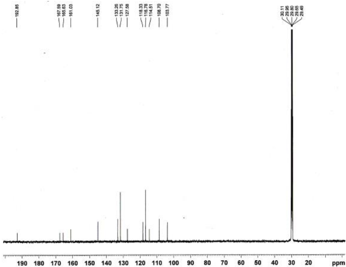
Figure S-2. ^{13}\text{C} NMR spectrum of isoliquiritigenin.
