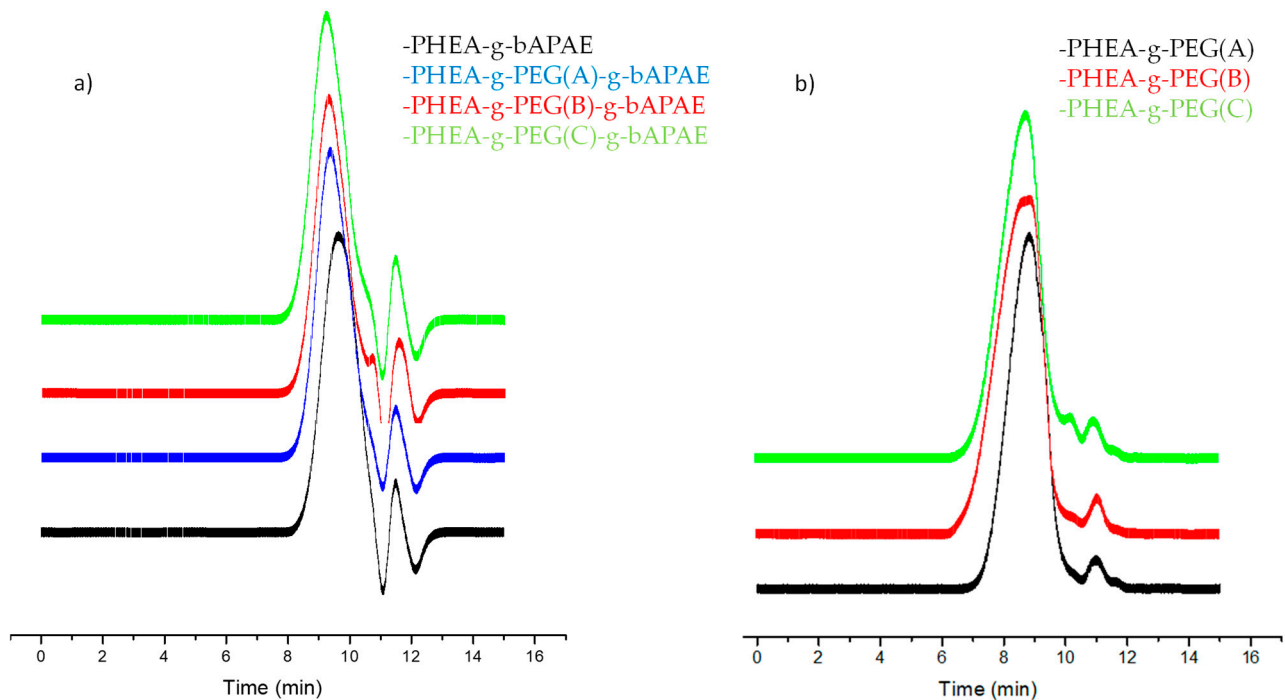
Figure S1. SEC chromatograms of: a) PHEA-g-bAPAE (black), PHEA-g-PEG(A)-g-bAPAE (blue), PHEA-g-PEG(B)-g-bAPAE (red), PHEA-g-PEG(c)-g-bAPAE (green); b) PHEA-g-PEG(A) (black), PHEA-g-PEG(B) (red), PHEA-g-PEG(C) (green).
