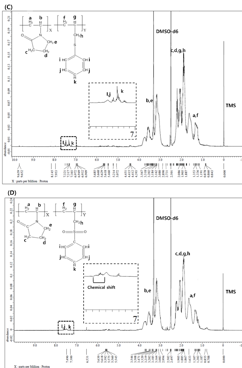
Figure S1. 1 H NMR spectrums of P(VP-APS)(97.5/2.5) (A), Oxi-P(VP-APS) (B), P(VP-APS)(96/4) (C), and Oxi-P(VP-APS)(96/4) (D).
