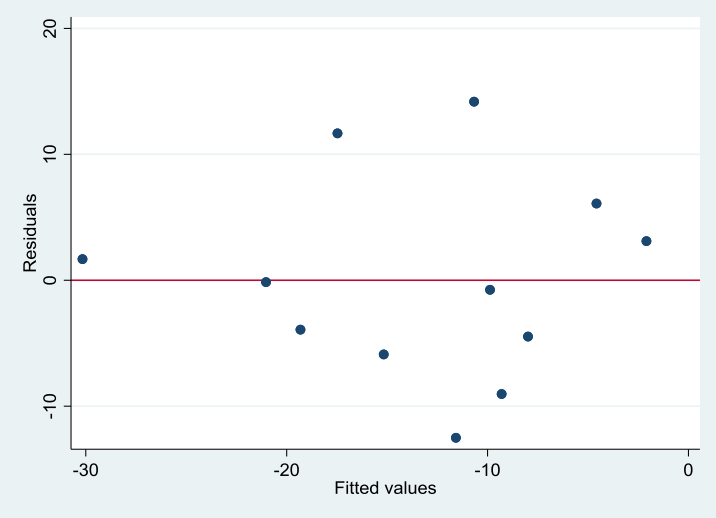
(C) Scatterplot of residuals vs fitted values
