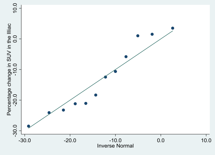
(A) Plot of normality
