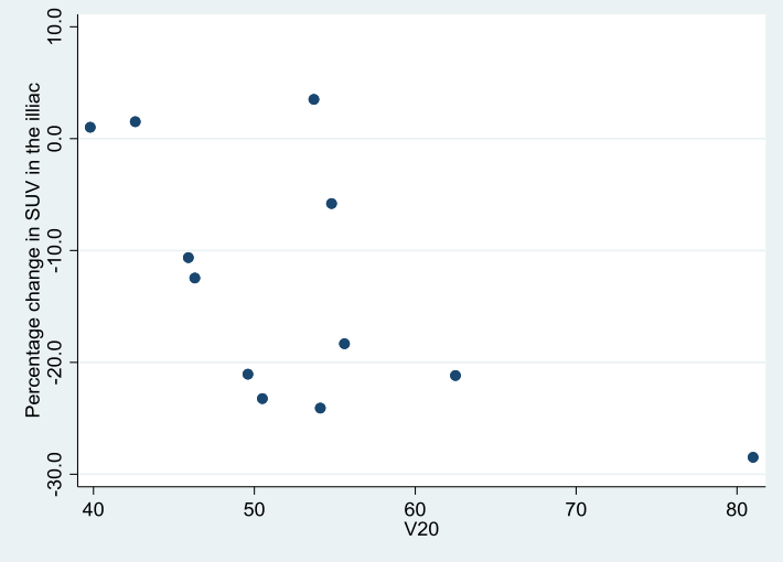
(B) Scatterplot of outcome vs predictor
