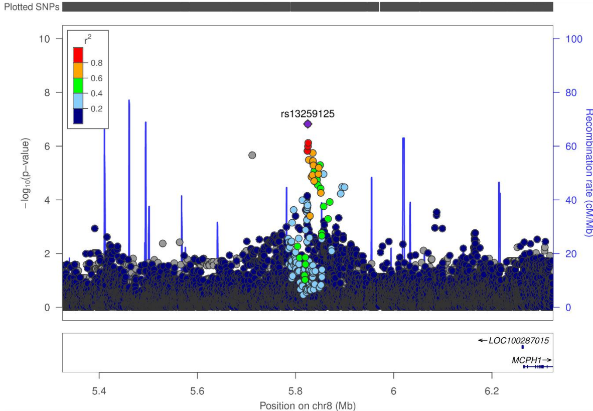
Supplementary Figure 7 Regional association plot for MCPH1 (rs13259125)
