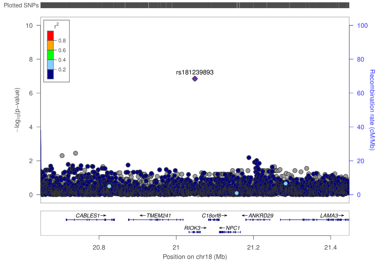
Supplementary Figure 5 Regional association plot for RIOK3 (rs181239893)
