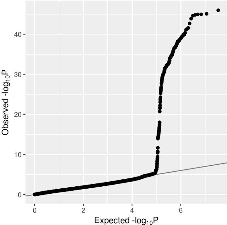
Supplementary Figure 2 Quantile-quantile plot for the sex-specific only analysis
