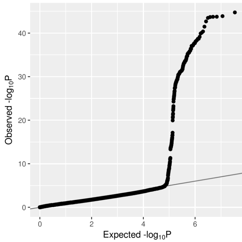
Supplementary Figure 1 Quantile-quantile plot for the joined FBAT-GEE analysis
