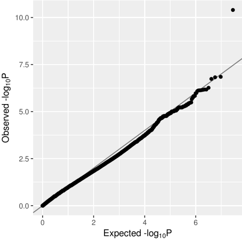
Supplementary Figure 3 Quantile-quantile plot for the sex-specific only analysis after additional quality control filtering
