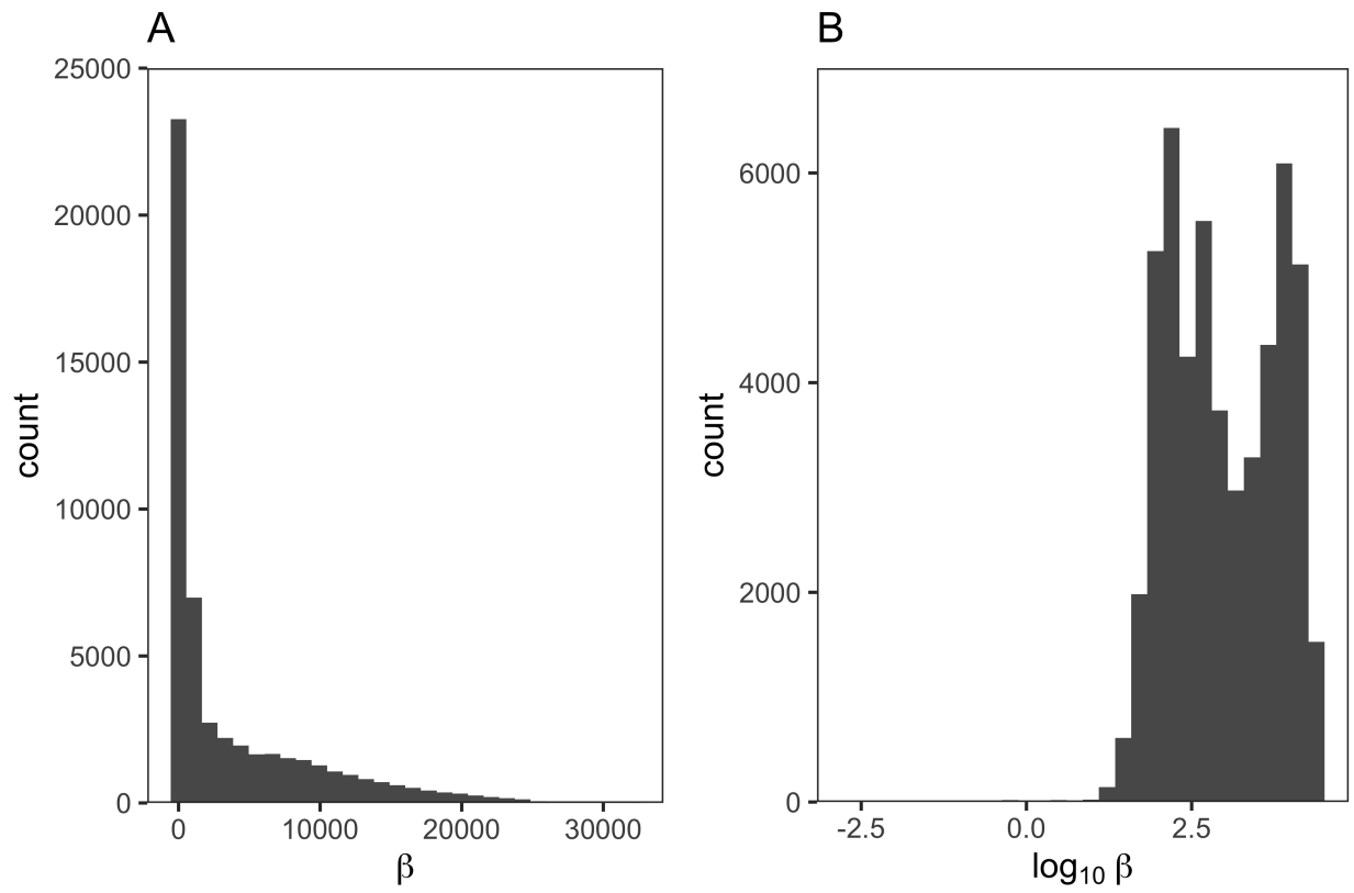
Figure S1: Histogram of (A) hyperpolarizability and (B) logarithmic transformation of hyperpolarizability.
