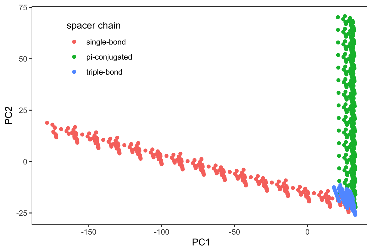
Figure S2: PCA plot based on the Klekota fingerprints for compounds containing single (red dots), alternating single/double (green dots), and single/triple (blue dots) carbon-carbon bonds
