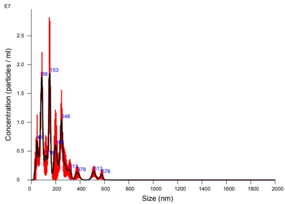
Supplementary Figure 1. Size distribution graph from nanoparticle tracking analysis (Nanosight NS01). Graph is the average of 3 x 30 sec flux at infusion of 40 \mu L/min into microfluidics chamber. Error bars indicate + / - 1 standard error of the mean.
