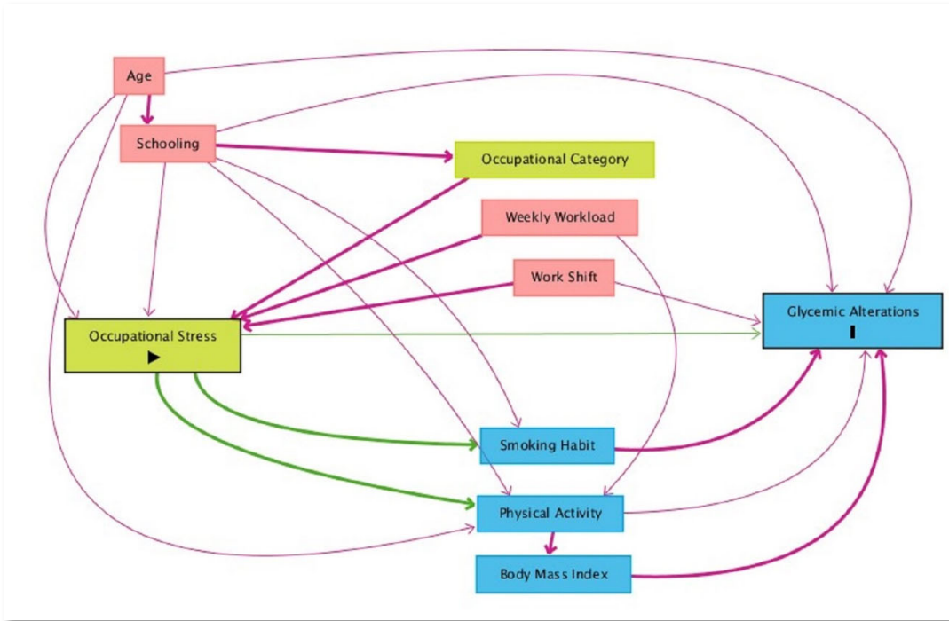
Figure S1. Directed Acyclic Graph (DAG) representing the association between Occupational Stress and glycemic alterations.
