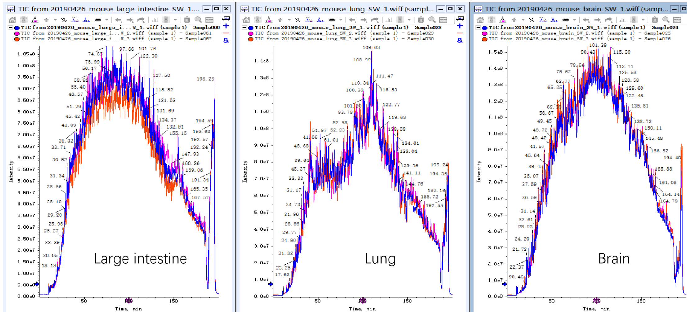
Supplementary Figure 2. The overlay of total ion chromatography (TIC) for three SWATH-MS runs in large intestine, lung and brain dataset.
