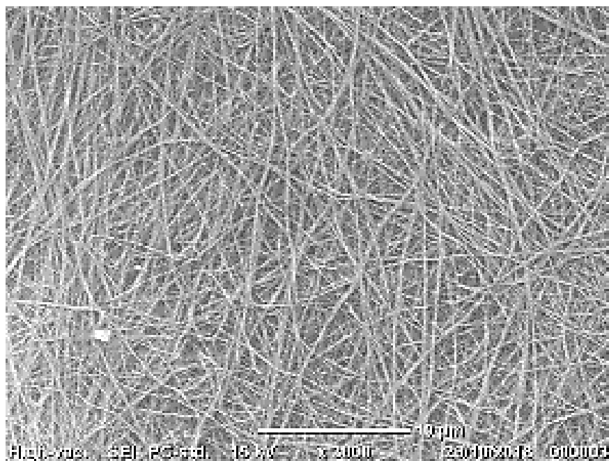
Supplementary figure 2. Scanning electron micrograph of the collagenous fibers composing the thermoresponsive hydrogel in figure S1.
