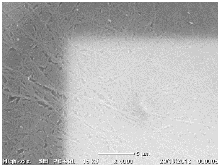
Supplementary figure 3. Scanning electron micrograph showing a large drug release electrode embedded within the thermoresponsive hydrogel.
