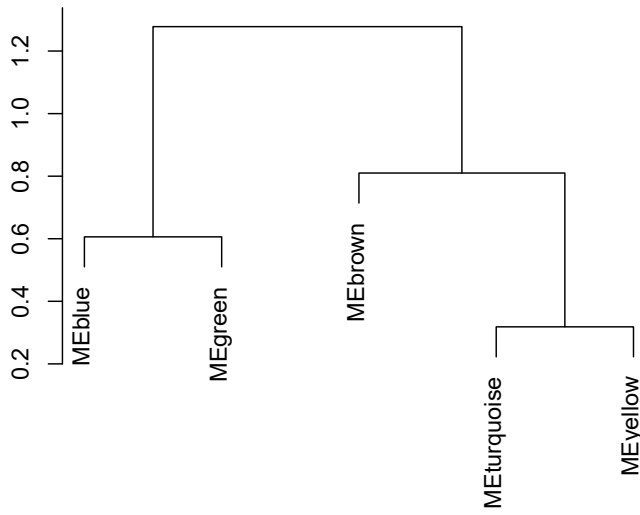
Eigengene dendrogram
