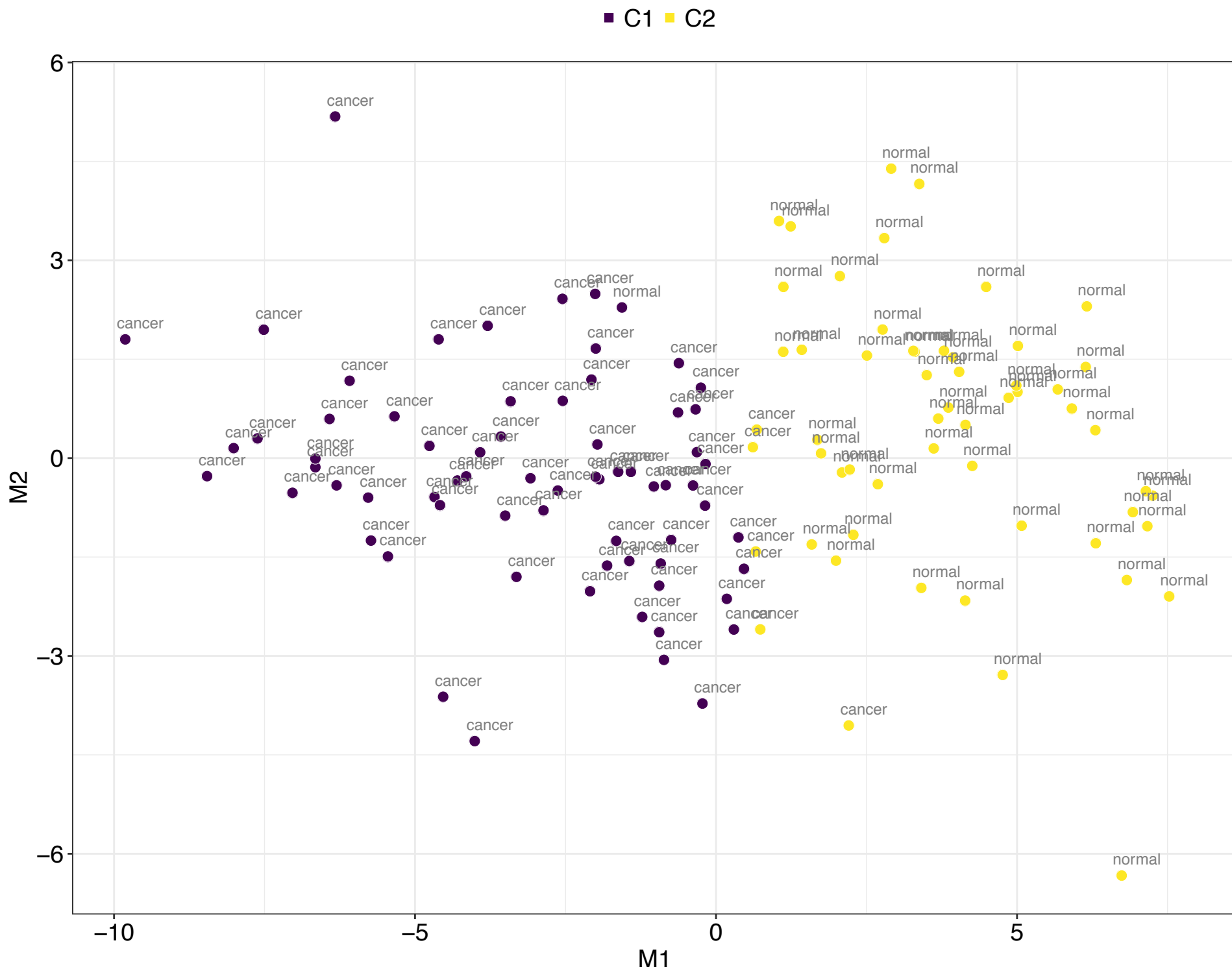
Supplementary Figure 1: Multidimensional scaling plot showing the result of k-means clustering with k = 2 . The two clusters support the anticipated difference between N-glycan abundances in normal interstitial fluid vs tumour interstitial fluid samples.
