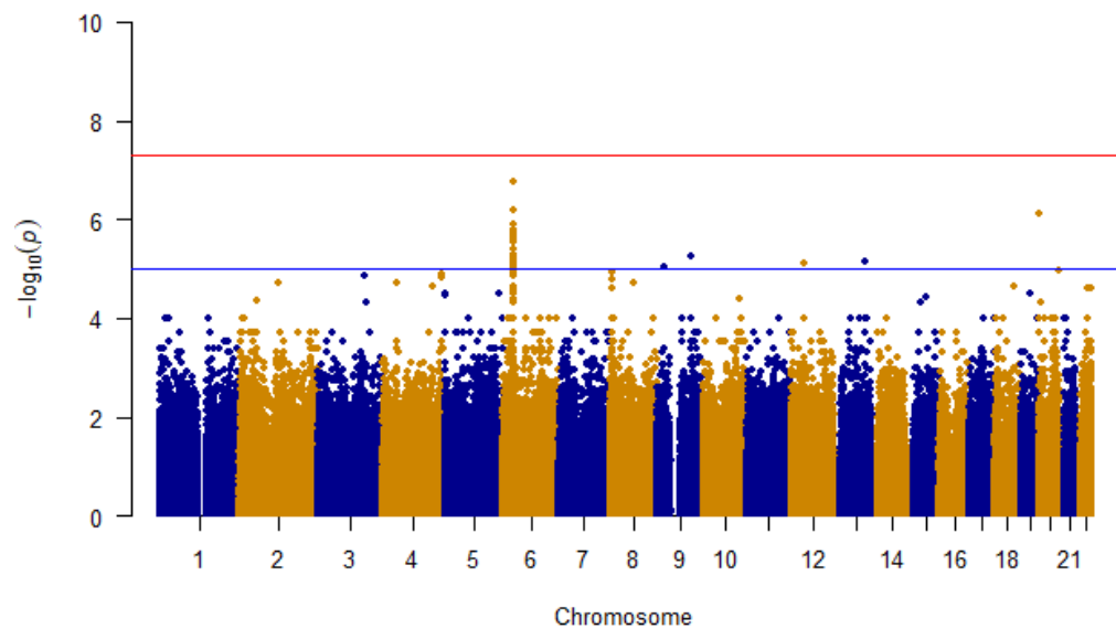
GeneMSA GWAS of 2009 SNP-level Manhattan Plot
