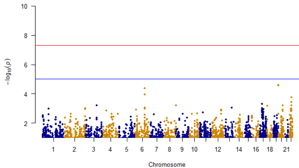
GeneMSA GWAS of 2009 Gene-level Manhattan Plot
