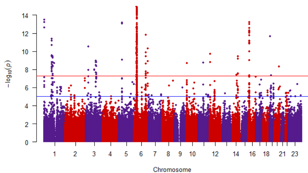
IMSGC GWAS of 2011 SNP-level Manhattan Plot
