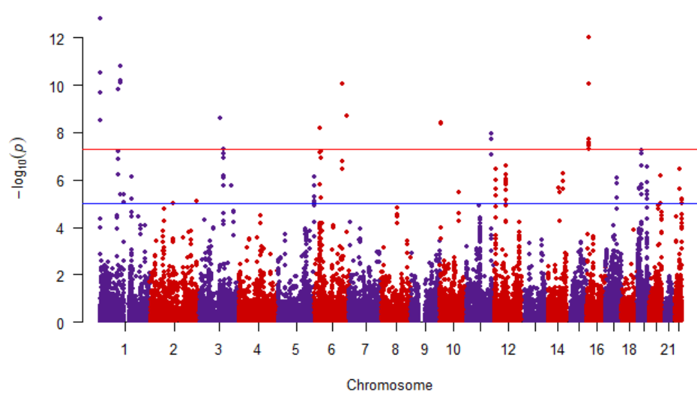
IMSGC GWAS of 2011 Gene-level Manhattan Plot
