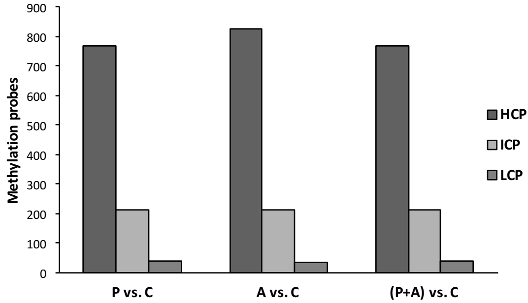
'00' methylation profile
