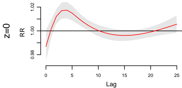
(a) Relative risk across lags
