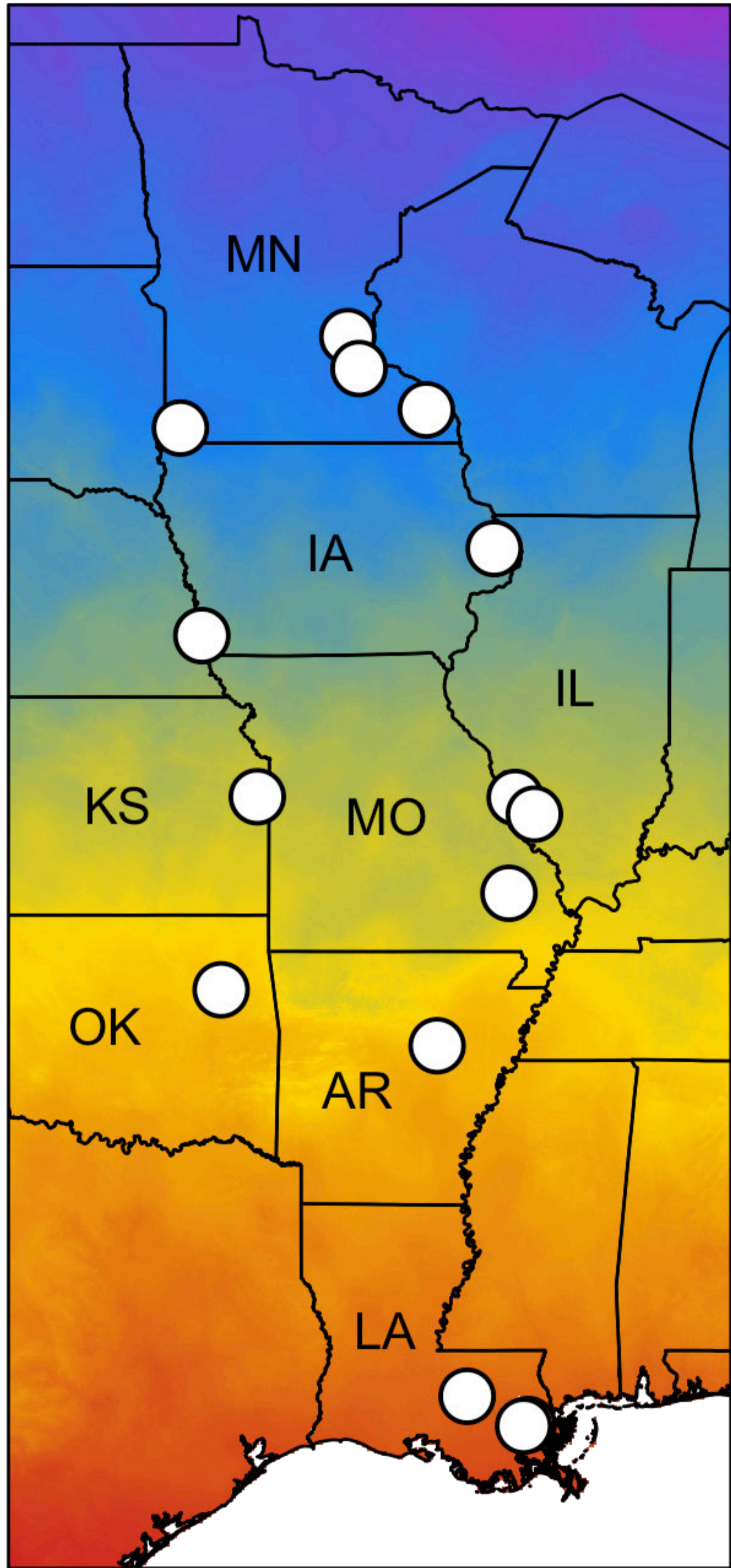
Annual mean temperature ( ^{\circ}\text{C} )
