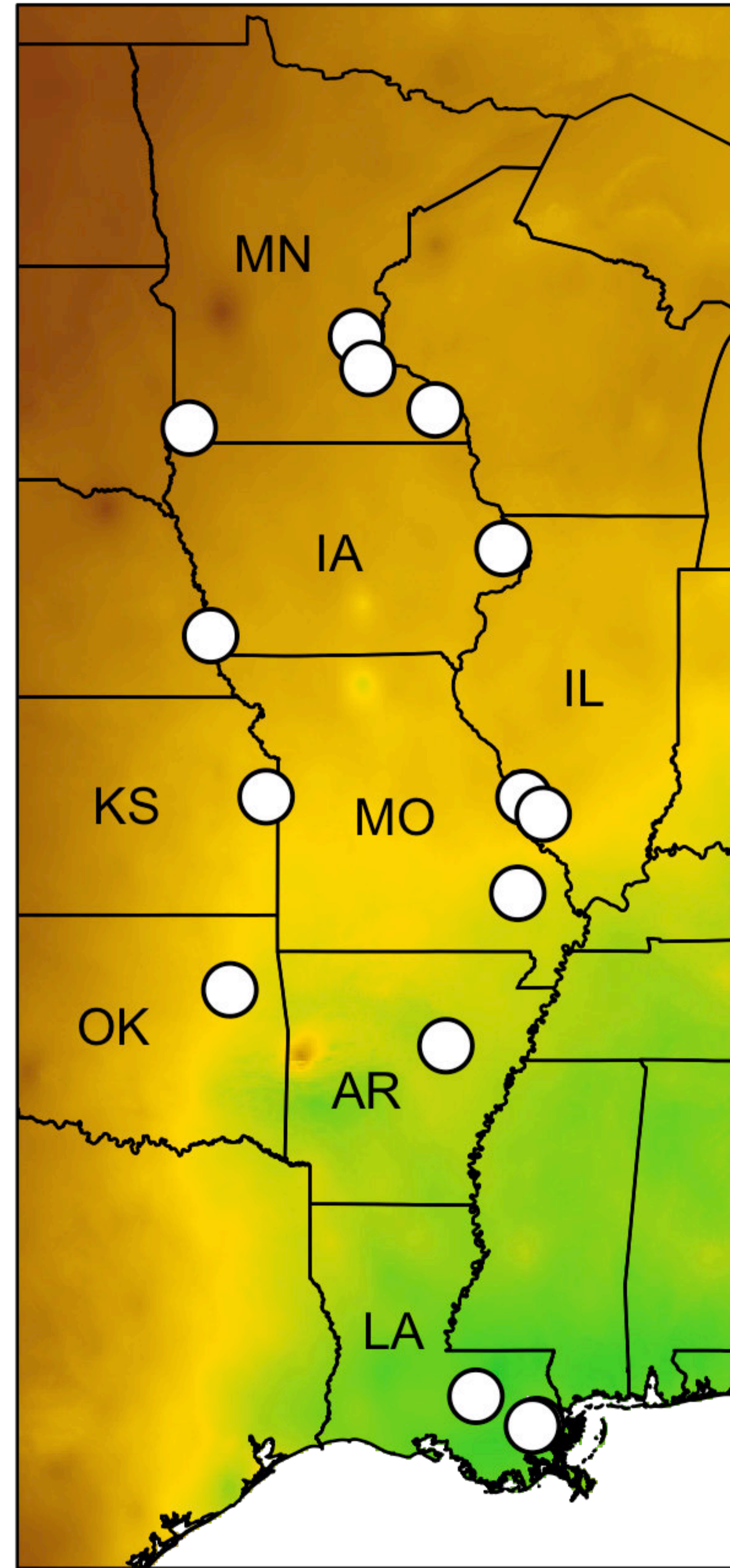
Annual precipitation (cm)
