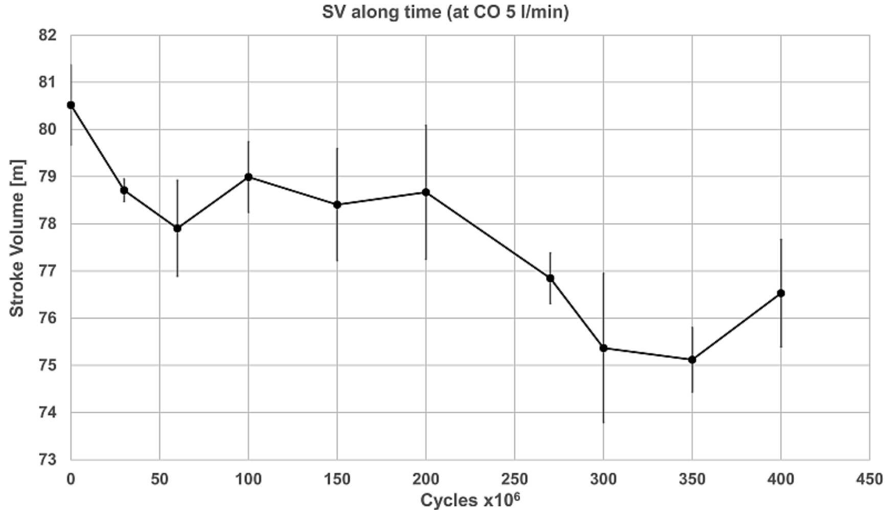
Supplementary Figure 1. Hydrodynamic performance of the polymeric valves along the AWT – complementary to Figure 4, showing the SV measured in the hydrodynamic testing along time in the AWT for constant CO of 5 L/min. AWT – Accelerated Wear Testing; CO – Cardiac Output; SV – Stroke Volume.
