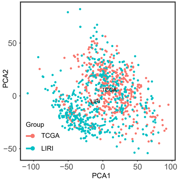
After removing batch effect
