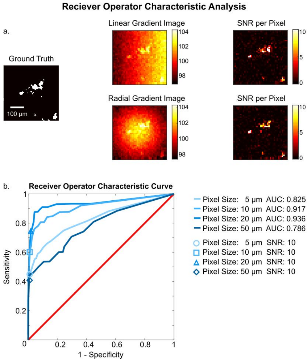
Figure 1. Receiver Operator Characteristic at various spatial resolutions. (a) The SNR of each pixel with linear and radial low frequency noise (b) ROC curve demonstrating poor detector ability at high and low spatial resolution (Pixel Sizes 5 \mu\text{m} , 50 \mu\text{m} ) and improved ability at optimized spatial resolutions (Pixel sizes 10 \mu\text{m} , 20 \mu\text{m} ).
