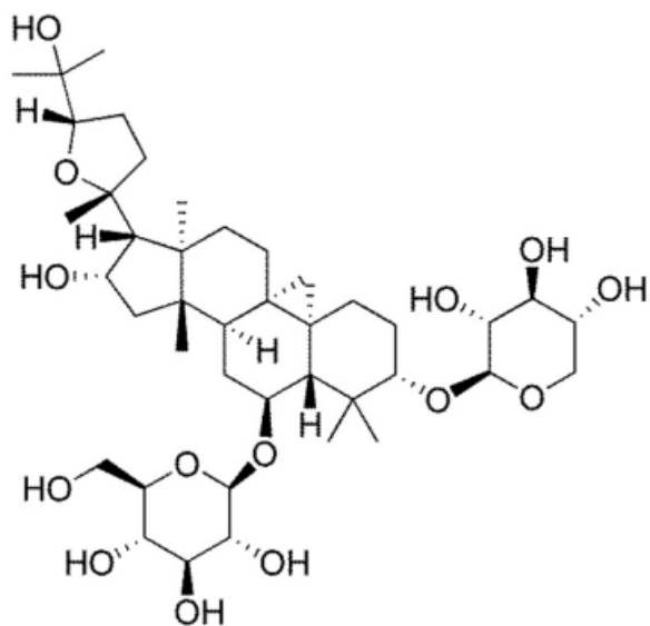
Supplementary Figure 1. The chemical structure of AST 1
