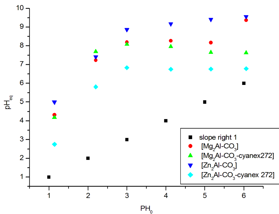
Figure S1. Variation in pH using the impregnated and non-impregnated LDH materials for zinc removal from aqueous solutions
