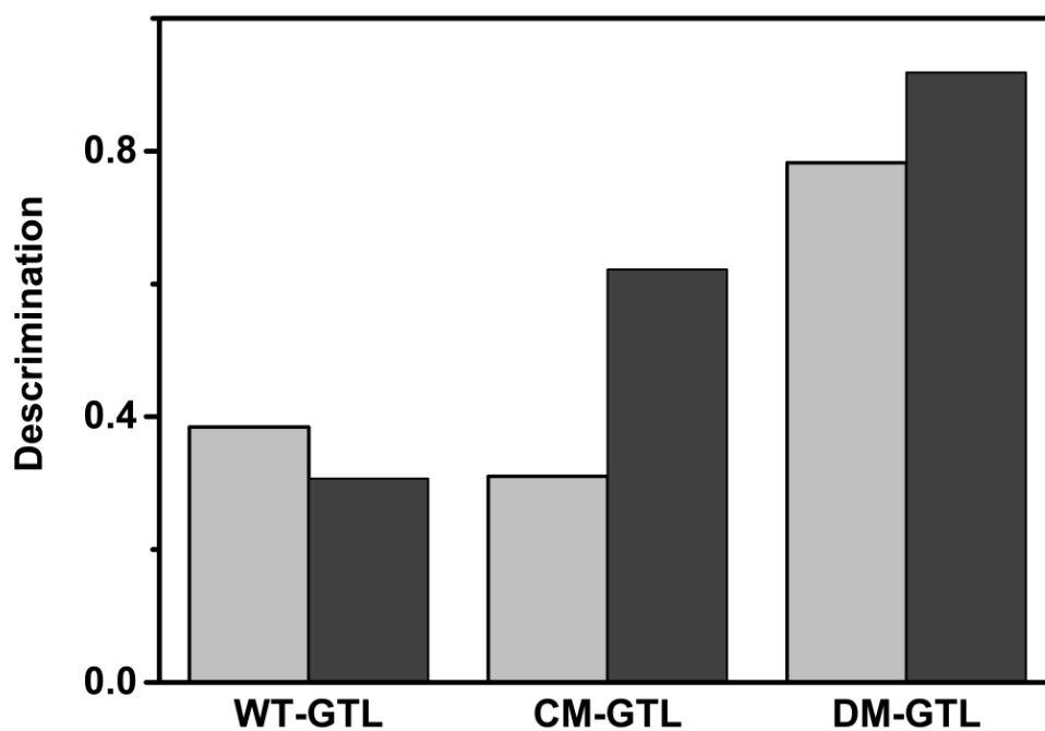
Figure S3: Fatty acid discrimination of GTL, CM-GTL and DM-GTL at 20 percent hydrolysis. EPA (Light grey) and DHA (Dark).
