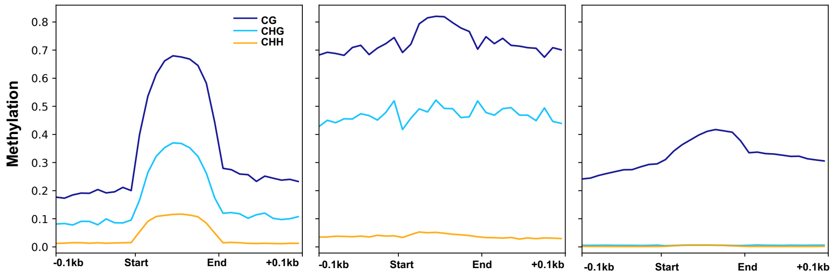
Heterochromatic intron without repeat
