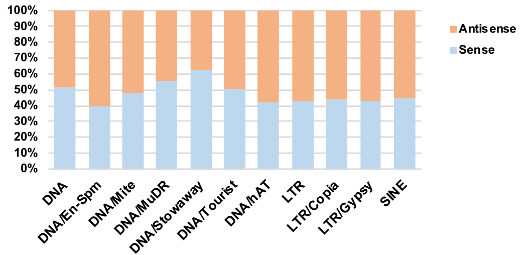
Orientation of intronic TEs against genes
