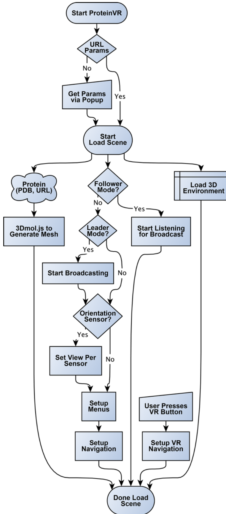
S1 Fig. Flowchart diagram representing the main steps of the ProteinVR algorithm. Oval nodes representing starting and stopping points. Diamonds represent decision points. Trapezoids represent points of manual input. The cloud represents data loaded from a remote source. The partitioned rectangle represents data loaded from within the ProteinVR app itself (internal storage). Plain rectangles represent algorithmic process steps.
