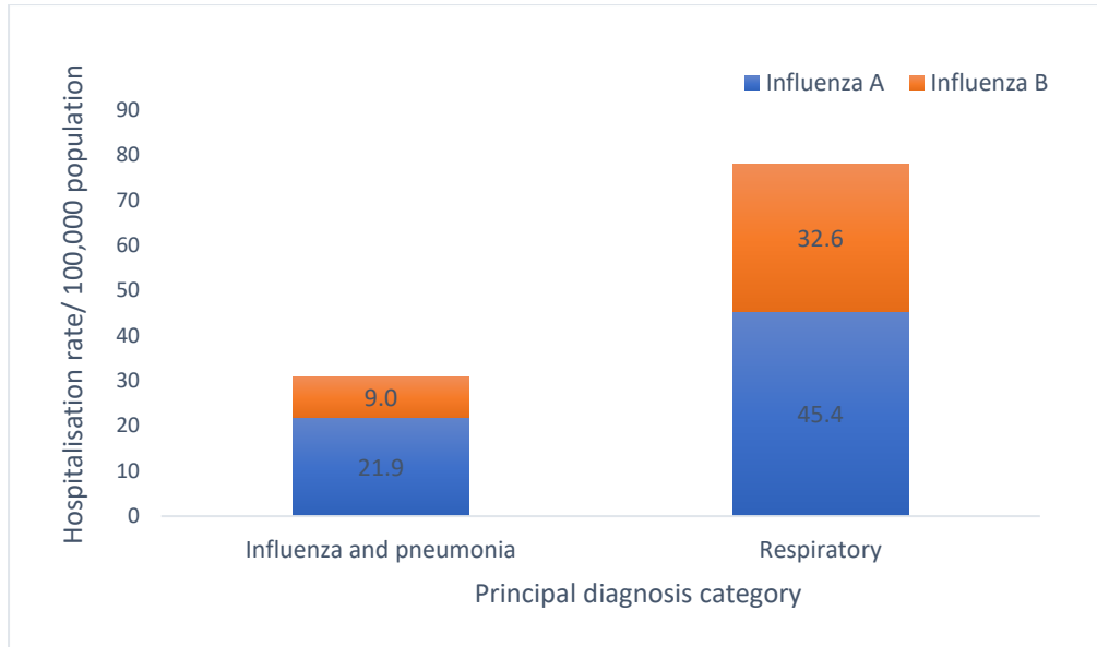
Figure S1. Estimated, all-age average annual rates of influenza-attributable hospitalisations, by diagnosis category using influenza A and B model
