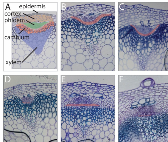
Figure S2. Histological analysis of the stem base of rev5 and wox4 mutant plants. A , Schematic overview of the arrangement of vascular tissue in the Col-0 wild type plant. B , Col-0 wild type, C , 35S::WOX4 , D , wox4 , E , rev-5 , F , wox4 rev-5 double mutant plants grown in log day conditions. Main stems of plants were sectioned after reaching a minimal height of around 10 cm. Highlighted in red is the cambial cell layer.
