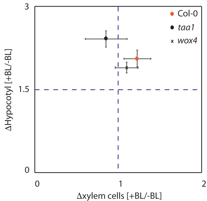
Supplementary Figure S11. Differential growth analysis of plants grown on medium +/- brassinolide. Diagram plotting the relative extension of the hypocotyl (y-axis; length of the hypocotyl in WL+BL divided by the length in WL-BL conditions) against the relative changes in TE cell number (x-axis; number of TE cells in WL+BL divided by the number of TE cells in WL-BL conditions) including the added standard errors.
