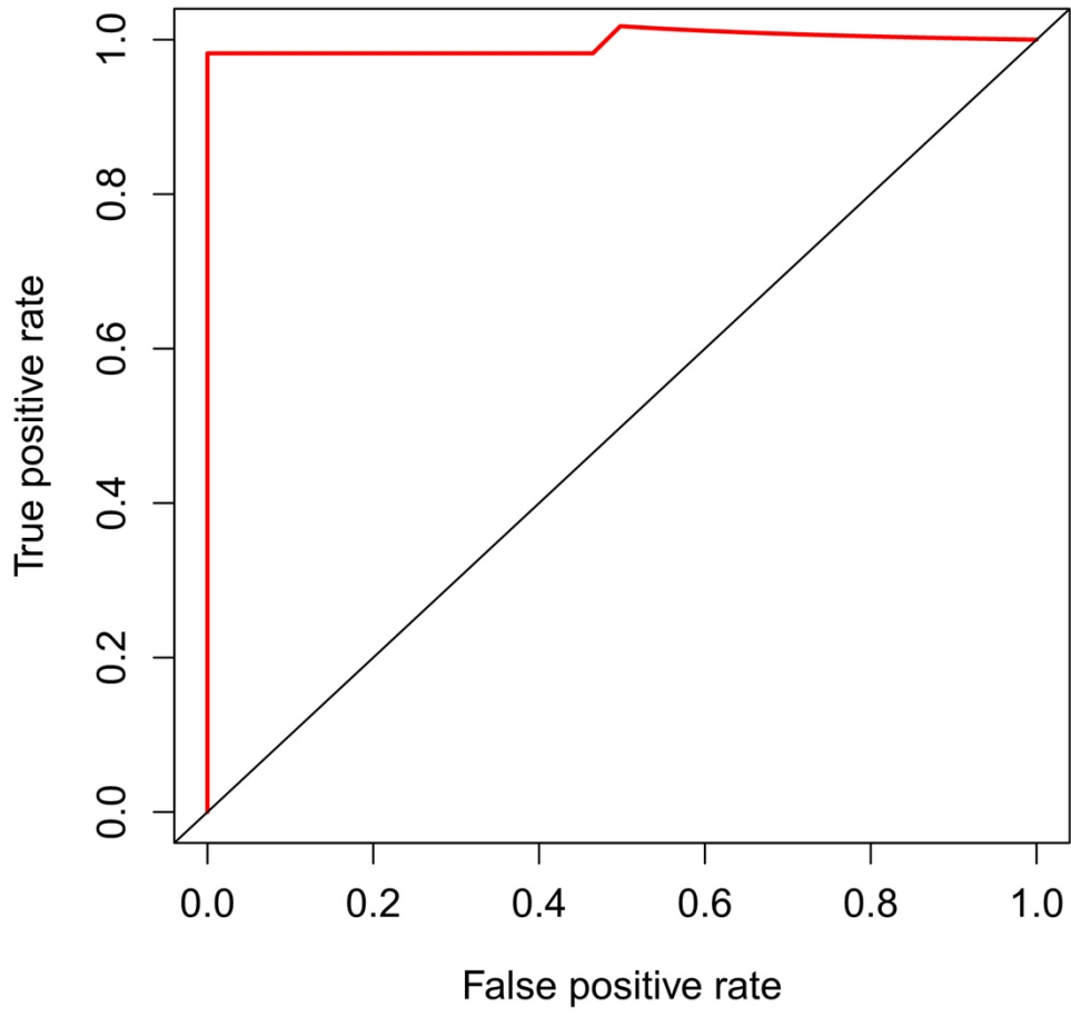
ROC curve ( AUC = 0.995 )
