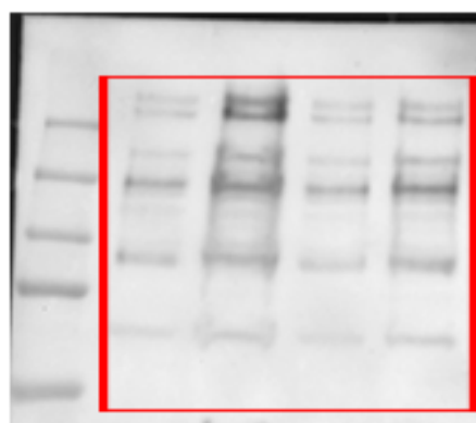
Figure 6B O-GlcNAc
