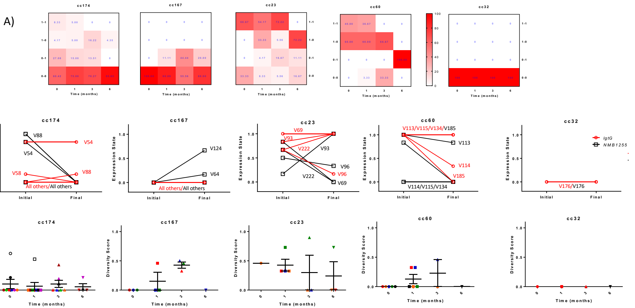
Supplementary Figure 6. Phasotypes for the LPS module ( IgtG and NMB1255 ). A) Percentages were calculated as described in Supplementary Figure 3 for the following numbers of isolates; cc174, 48, 40, 37, 23; cc167, 14, 18, 18, 15; cc23, 6, 24, 18, 18; cc60, 30, 30, 12, 6; cc32, 6, 6, 6, 6. B) Switching states for each volunteer for the LPS module. See Supplementary Figure 3 for method for determination of expression states. C) Shannon diversity scores for each time point. See Supplementary Figure 3 for how diversity scores were derived.
