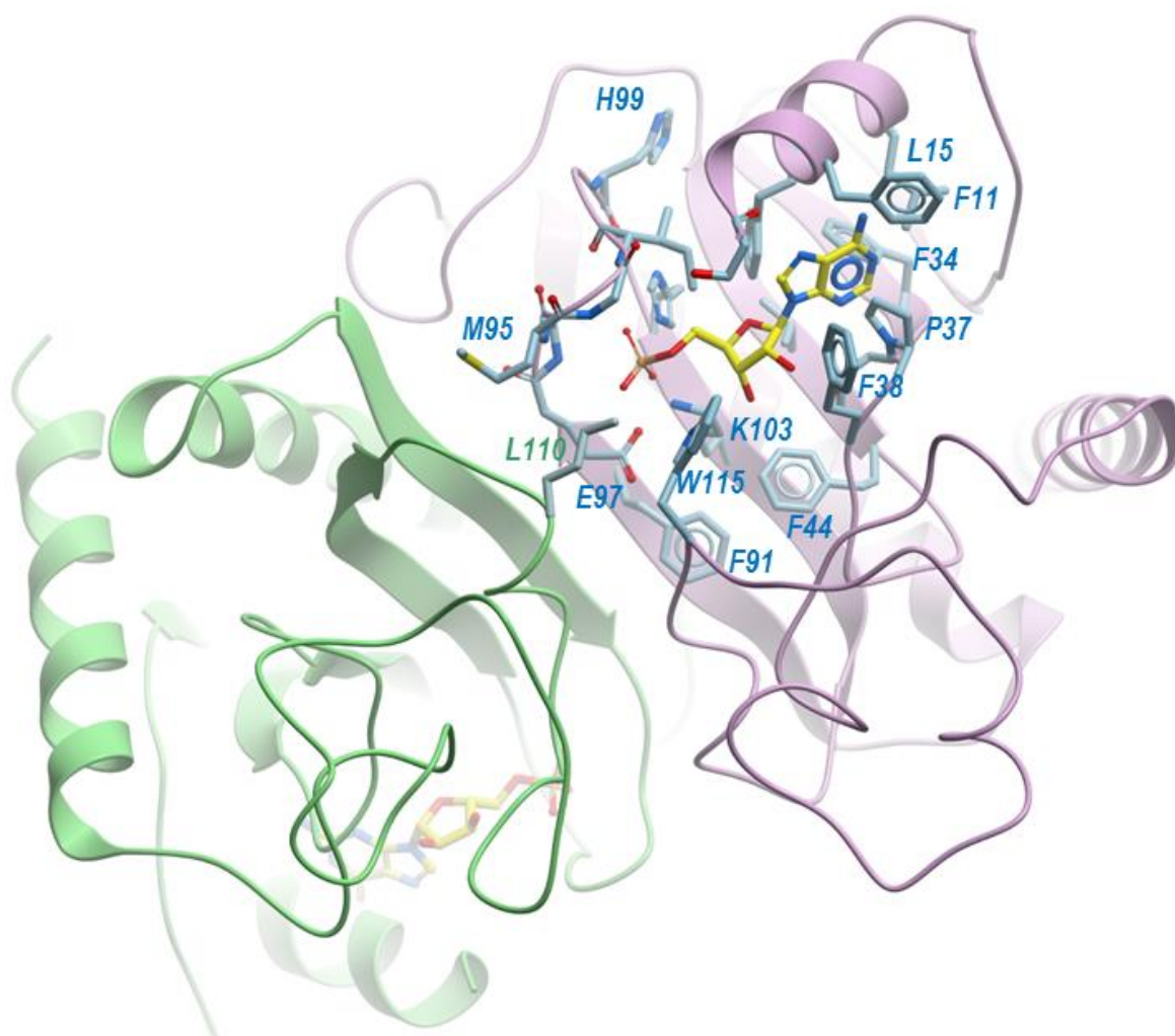
Figure S5. 3D-structural model of McchHmi dimer in complex with AMP. The two monomers of McchH are depicted as light green and purple colored ribbons diagrams. Residues of the active site that form the substrate-binding pocket are labeled and shown in a stick representation.
