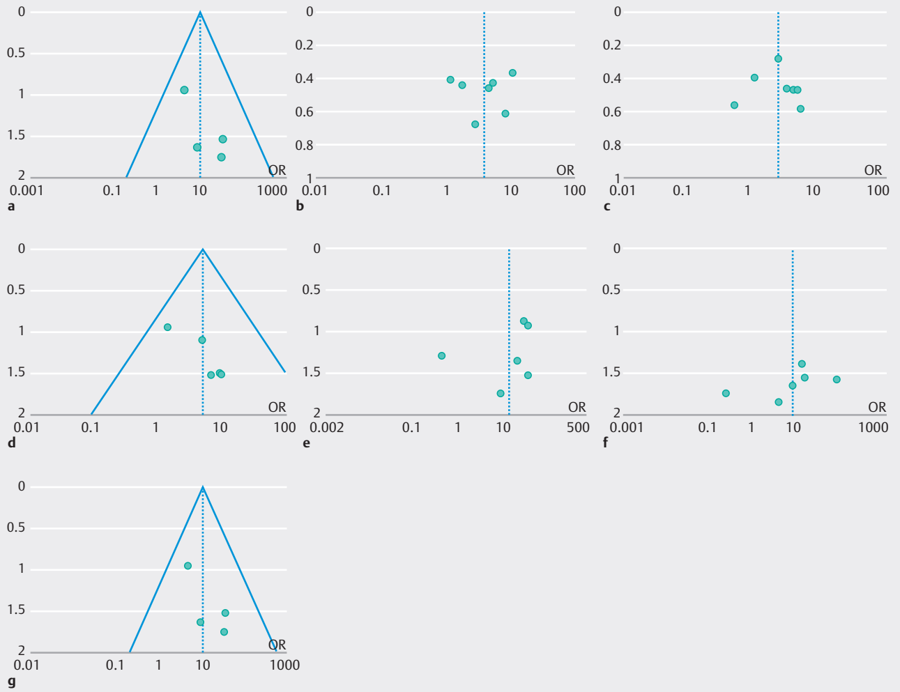
► Supplementary Fig. 9 Funnel plots for studies. a Diagnostic yield of TTNB histology vs FNA cytology for a specific cyst diagnosis. b Diagnostic yield of TTNB histology vs FNA cytology for mucinous cysts. c Diagnostic yield of TTNB histology vs CEA \geq 192 ng/mL for mucinous cysts. d TTNB histology vs FNA cytology for serous cystadenoma. e Concordance of TTNB histology vs FNA cytology with surgical pathology for a specific cyst type. f Concordance of TTNB histology vs FNA cytology with surgical pathology for a mucinous cyst. g Concordance of TTNB histology vs FNA cytology with histological severity on surgical pathology for a mucinous cyst.
