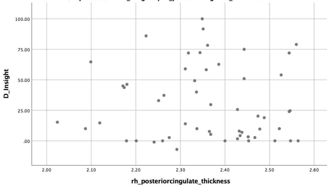
Simple Scatter of D_Insight by rh_posteriorcingulate_thickness
