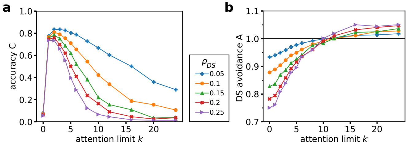
FIG. S5. Attention trade-off in a group of agents with active signalers. Each agent connected to another individual signalling direct interaction with a DS (direct responder), pays only attention to the signaller(s) and ignores other social cues. Accuracy C (a) and DS avoidance A (b) versus attention limit k for different DS densities at R_{inf} = 0.1 .
