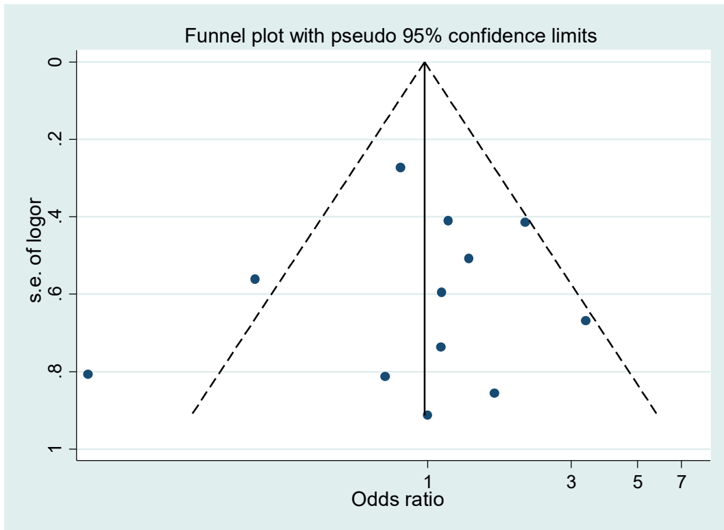
Funnel plot showing publication bias of 1-month mortality. Each point represents the odds ratio (OR) and the standard error of logOR for a single study.
