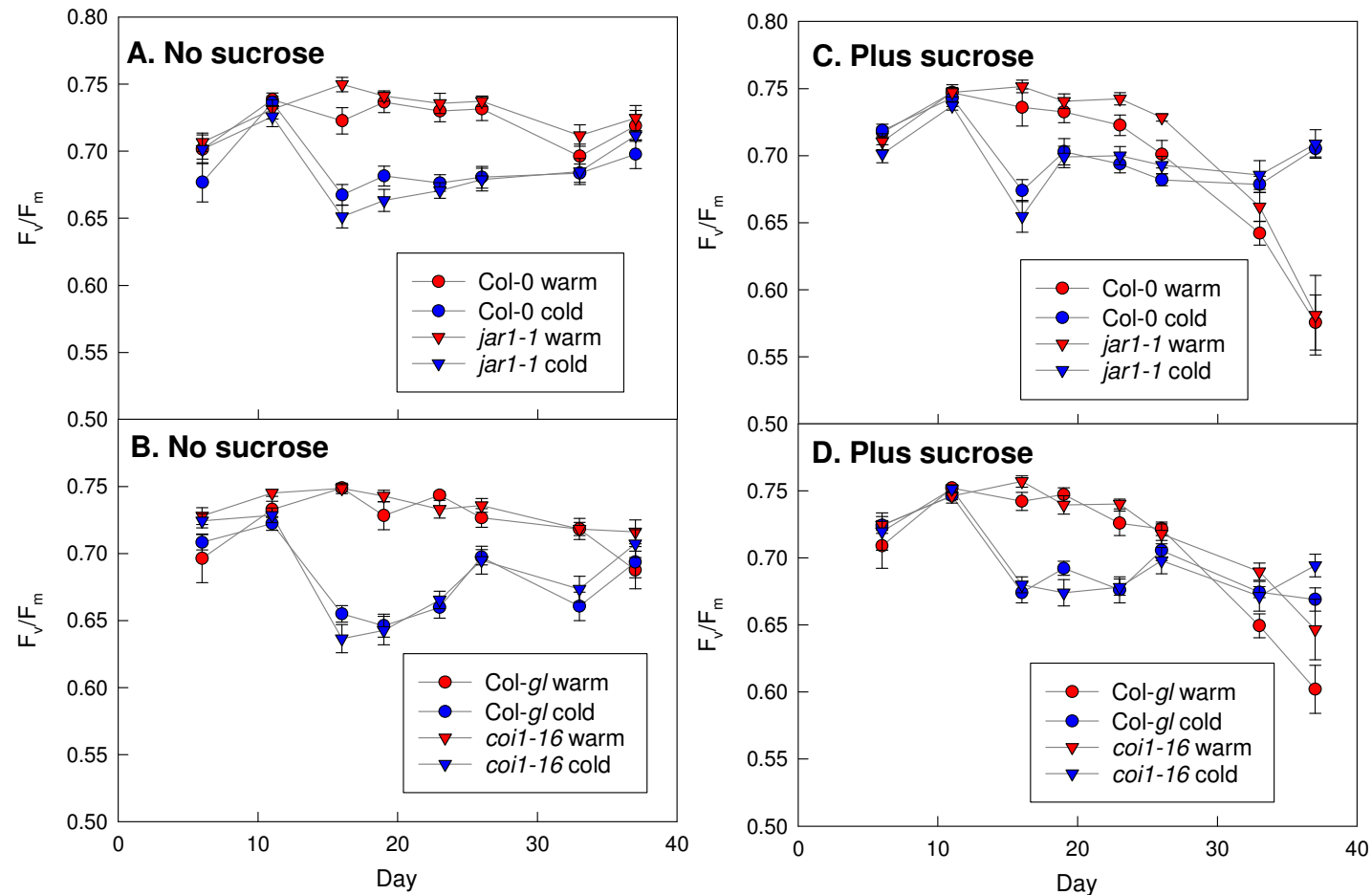
Additional file 2. Effect of cold treatment on F_v/F_m in the jar1-1 (A and C) and coi1-16 (B and D) mutants and their respective wild types, Col-0 and Col- gl . The plants were grown on agar plates without sucrose (A and B) or with addition of 55 mM sucrose (C and D). F_v/F_m was determined for the whole rosette by fluorescence imaging. The plates were incubated at 20°C until day 13 and then either kept at 20°C (red symbols) or transferred to 4°C (blue symbols) for the remainder of the experiment. Data are means of 5 plates \pm SE.
