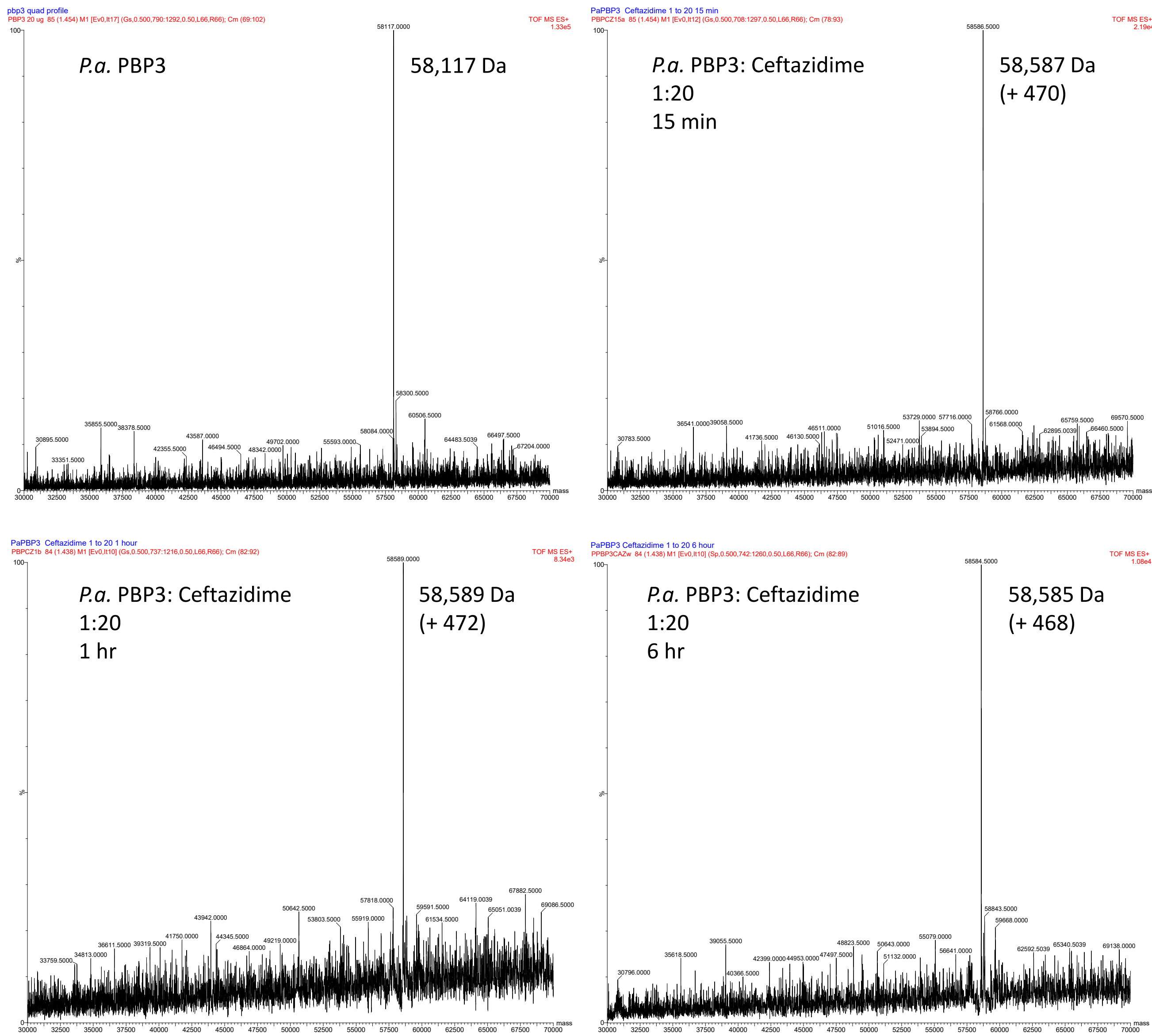
Mass spectra of P. aeruginosa PBP3 alone and after 15 min, 1 hr, and 6 hrs of preincubation with ceftazidime. P. aeruginosa PBP3/ceftazidime molar ratio is 1:20. Mass accuracy is \pm 5 Da.
