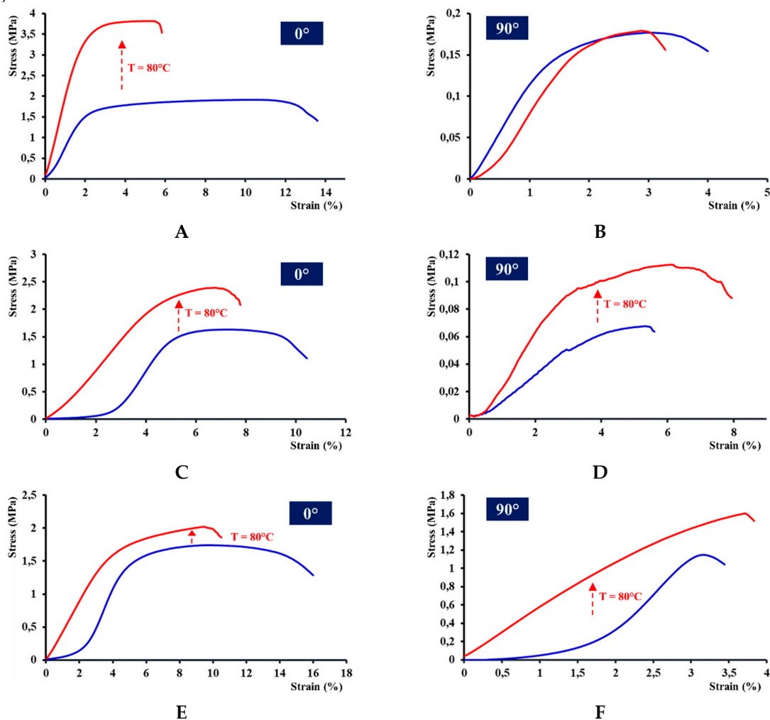
Figure S1. Stress–strain curves of the PHB/PCL mats before (blue) and after (red) thermal treatment onto rotating drum (A, B), blade (C, D) and grid (E, F) collectors at different directions of cutting.
