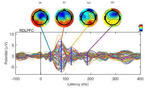
Topoplots of the corrected TEP of P008 (Avref)
