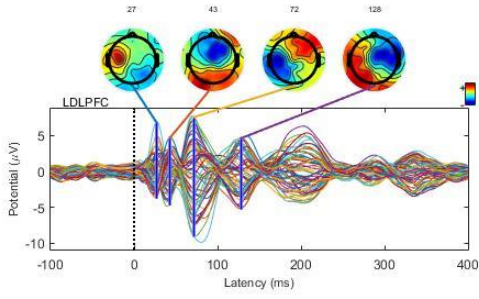
Topoplots of the corrected TEP of P008 (Avref)
