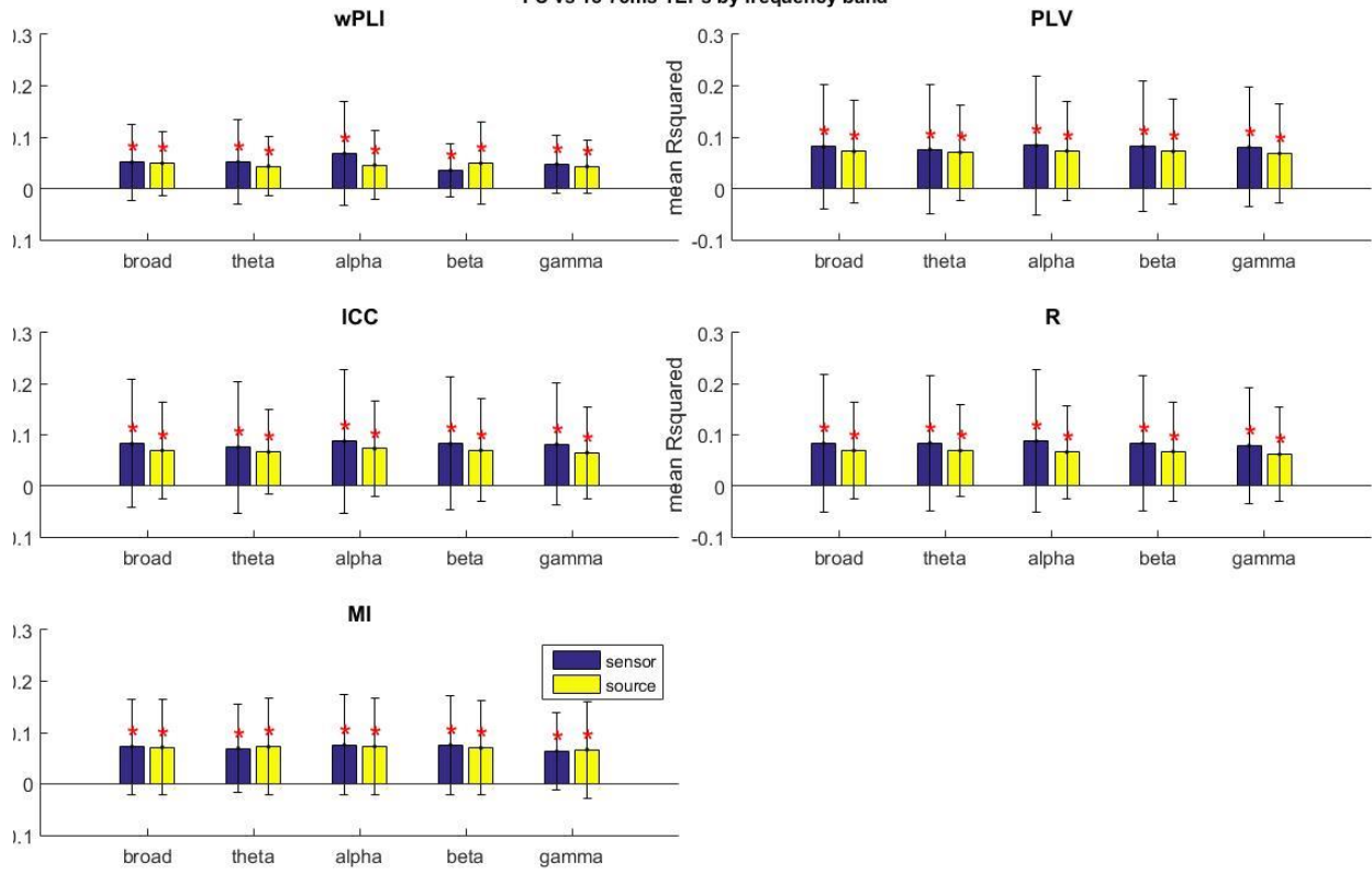
FC vs 15-400ms TEPs by frequency band
