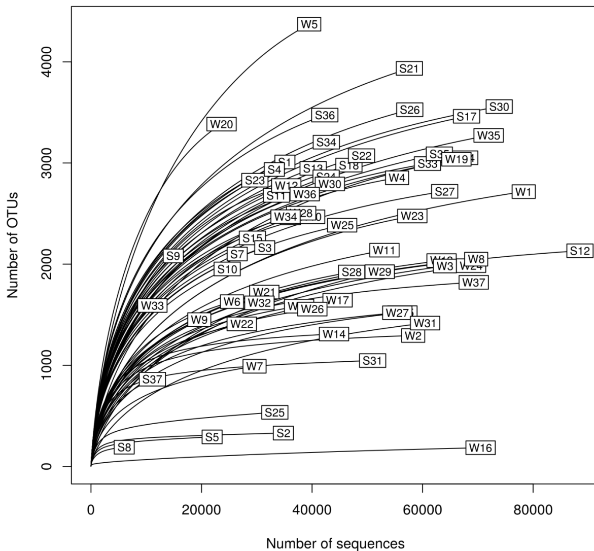
9 Figure S1. Rarefaction curves for the soil (S*) and aquifer (W*) samples.
