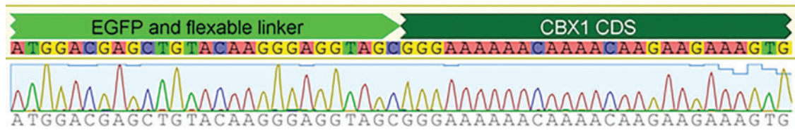
SUPPLEMENTARY FIG. S3. PCR amplicons eGFP-positive cells generated from MAD7 gRNA1 were cloned and Sanger sequenced at each eGFP insertion junction.
