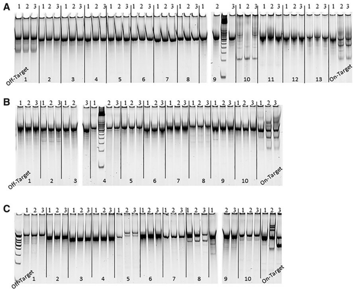
SUPPLEMENTARY FIG. S8. DNA mismatch detection assays using Cel-I enzyme for predicted off-targets. (A) PCR amplification products from predicted off-targets for the mouse Rosa26 gRNA #1 used in a DNA mismatch detection assay with the Cel-I enzyme. (B) Mouse Rosa26 gRNA #2 predicted off-targets in the same assay as in A above. (C) Rat Calb2 gRNA #1 predicted off-targets in the same assay as in A above. WT (#1), an individual indel sample (#2) and pool of all the positive indel samples (#3). On-target represents the designed and intended mouse or rat target, respectively. Unlabeled and banded lanes represent DNA markers, unlabeled in this case.
