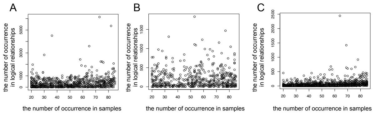
Fig. S3 Relationships between the number of occurrence of the item in the dataset and those in the detected logic relationships for (A) eggNOG ortholog dataset, (B) KEGG OC ortholog dataset and (C) OTU dataset. The x-axis and the y-axis represent the number of occurrence of the item in the dataset and that in the detected logic relationships, respectively.
